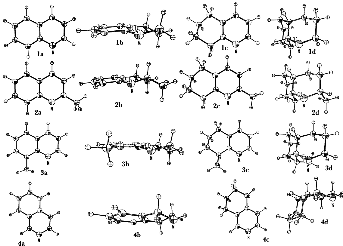
Fig. 5. Structure models of related compounds. See Table 3 for the chemical names of symbols.
